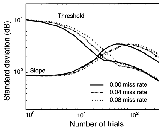
Fig. 3. Performance of the \Psi method with assumed miss rates of 0, 0.04 and 0.08. The miss rate for the simulated observer matched the assumed miss rate of the method. The assumed value of the miss rate greatly affects the method efficiency.
